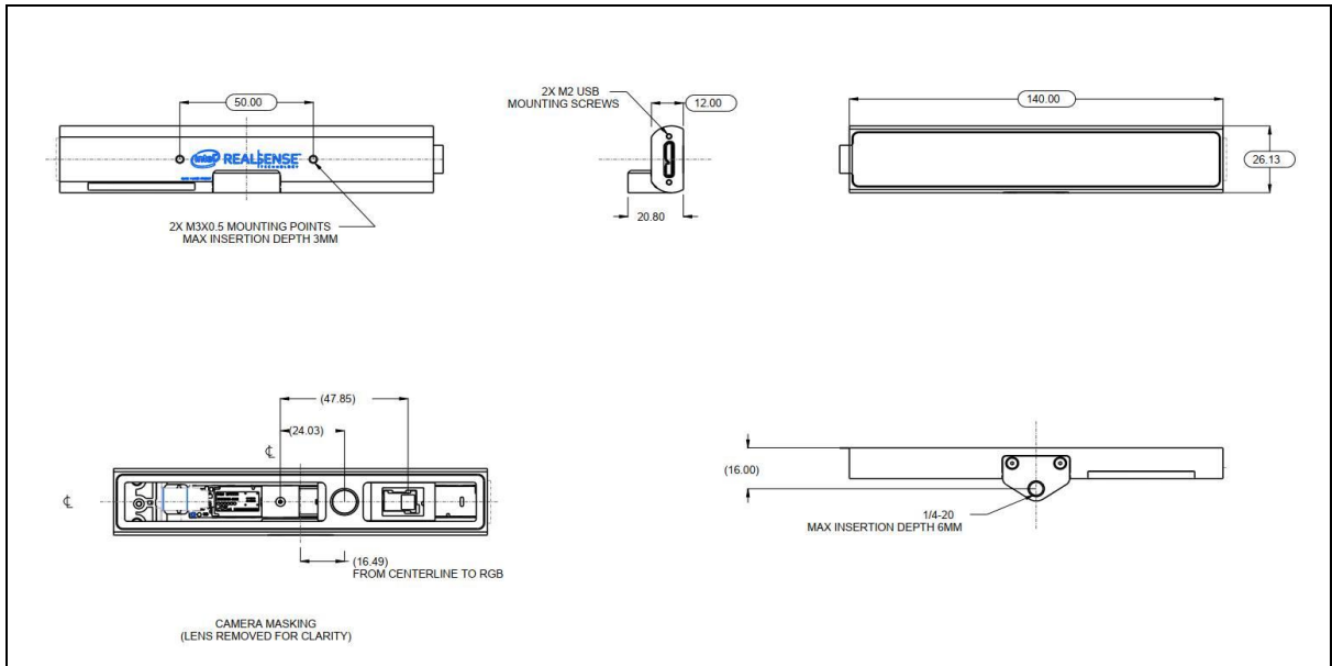
Figure 9-2. Intel® RealSense™ Depth Camera SR305
